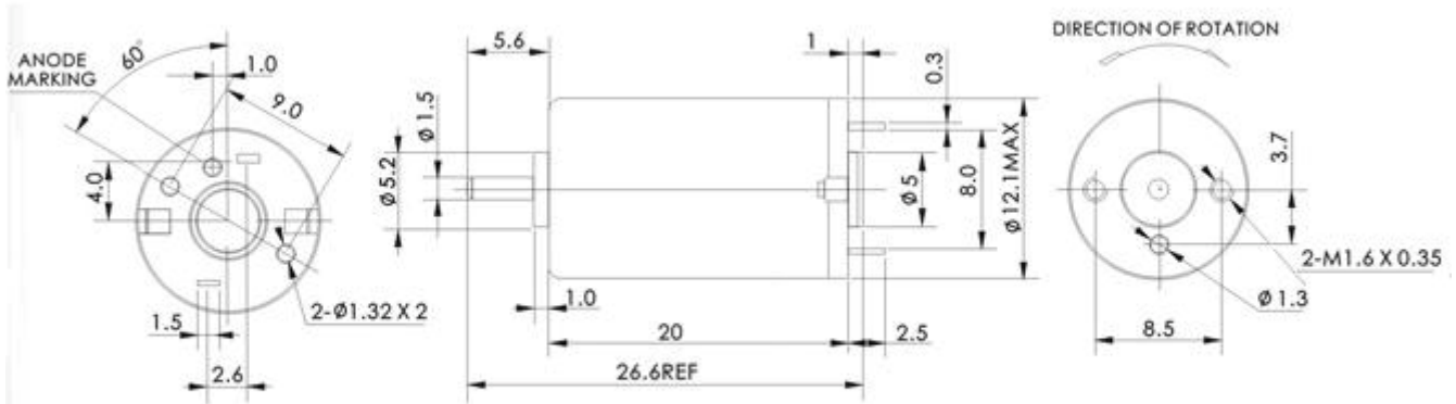
UNIT : Millimeters WEIGHT : 8 g (APPROX)
