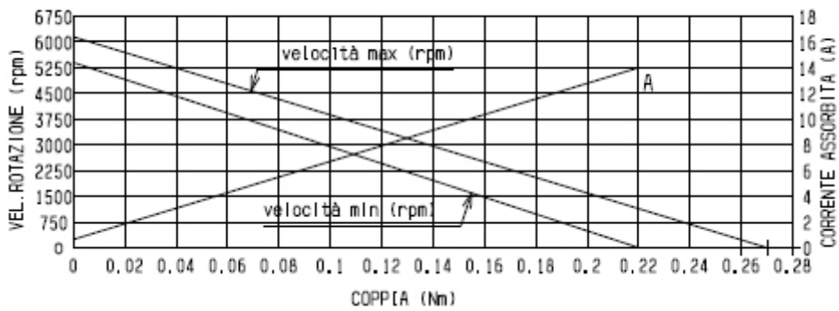
CURVE CARATTERISTICHE 13.5 V RESIST.LINEA 0.15 ohm (B)
