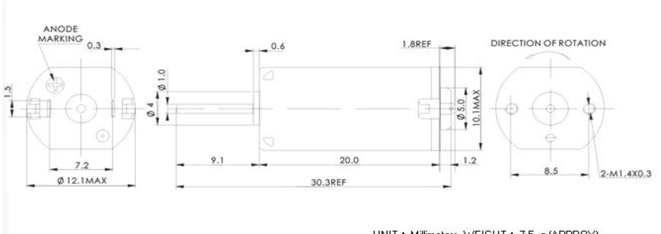
UNIT : Millimeters WEIGHT : 7.5 g (APPROX)
