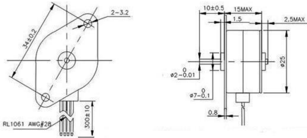
UNIT : Millimeters WEIGHT : 80 g (APPROX)
